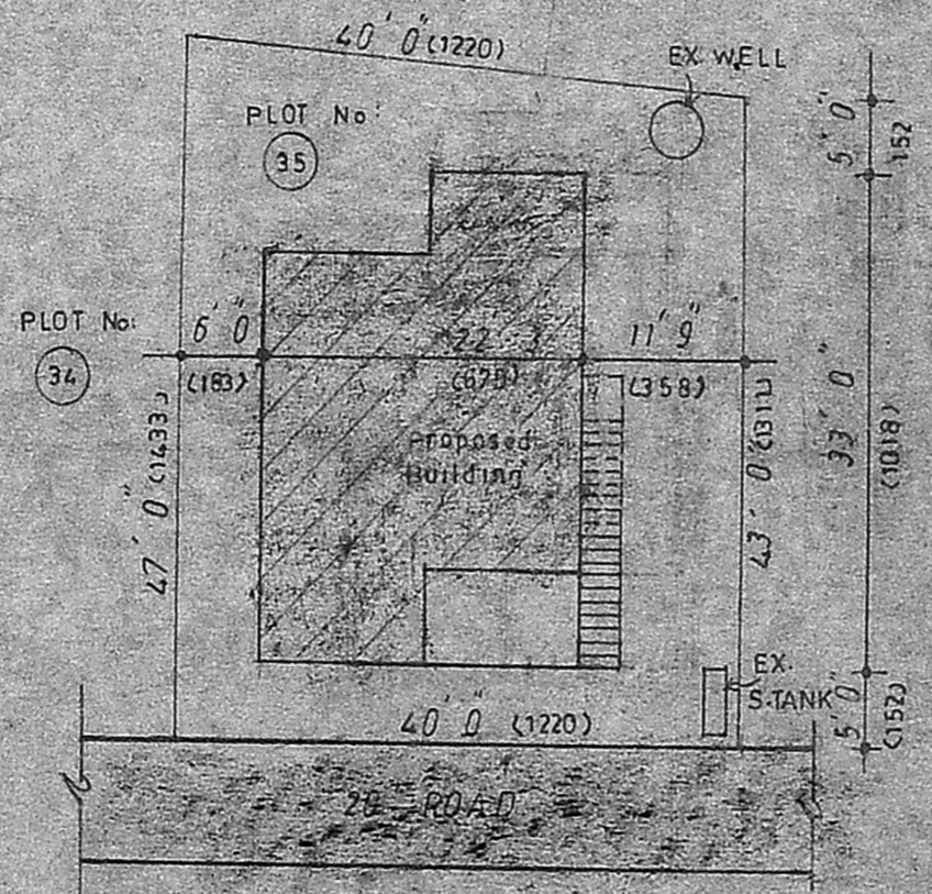
site plan
